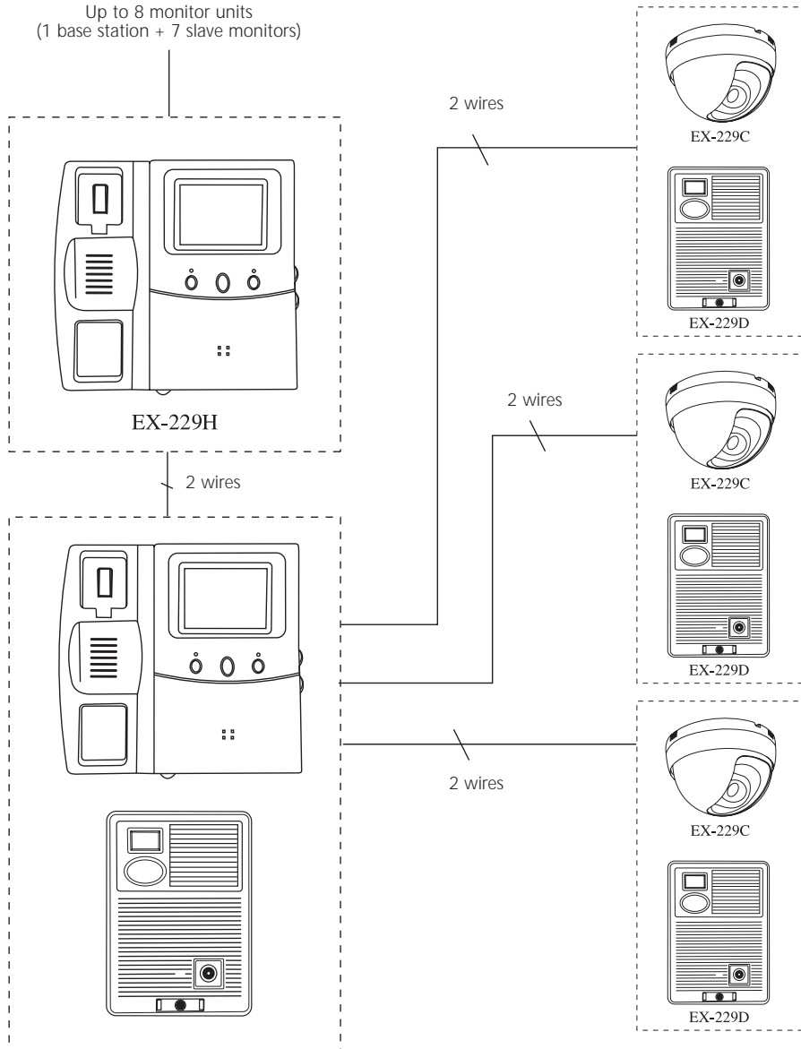
M229 - DOORPHONE SYSTEM
