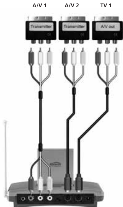
Figure 1 A/V TRANSMITTER
