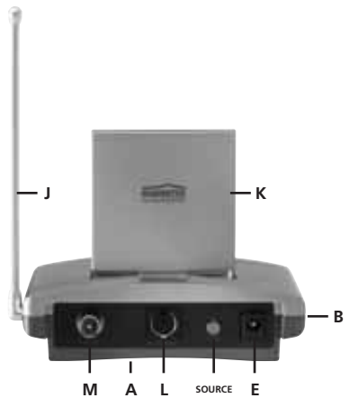
Figura 4 RECEPTOR A/V
