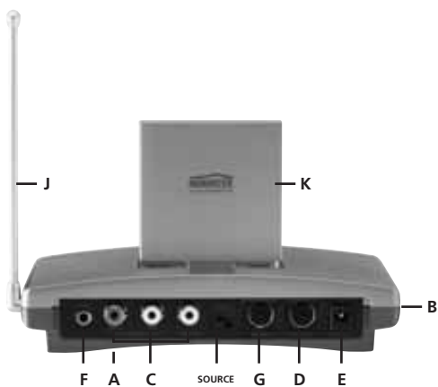
Figure 3 A/V TRANSMITTER
